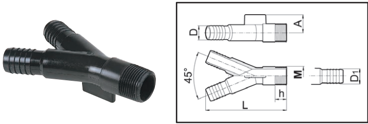
Raccordi a "Y" "Y" fitting Racor en "Y"
